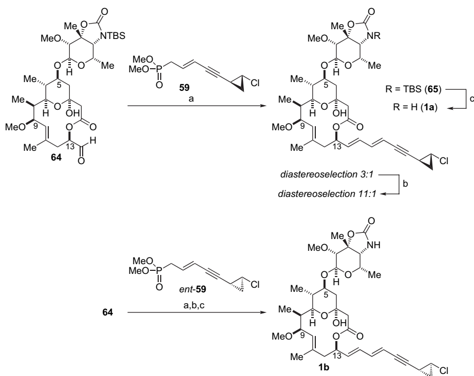
Scheme 21. Reaction conditions: (a) LiHMDS, −78 °C to rt; (b) I 2 , CH 2 Cl 2 , rt; (c) TBAF, AcOH, THF, rt, 56% (for 1a ) and 43% (for 1b ) from alcohol 63 .
