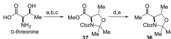
Scheme 11. Reaction conditions: (a) NaOH, CbzCl, MeCN, \text{H}_2\text{O} ; (b) MeI, \text{K}_2\text{CO}_3 , DMF; (c) TsOH, \text{Me}_2\text{C}(\text{OMe})_2 , acetone, 93% (three steps); (d) ^i\text{PrMgCl} , MeONHMe·HCl, THF, 93%; (e) MeMgBr, THF, 69%.
