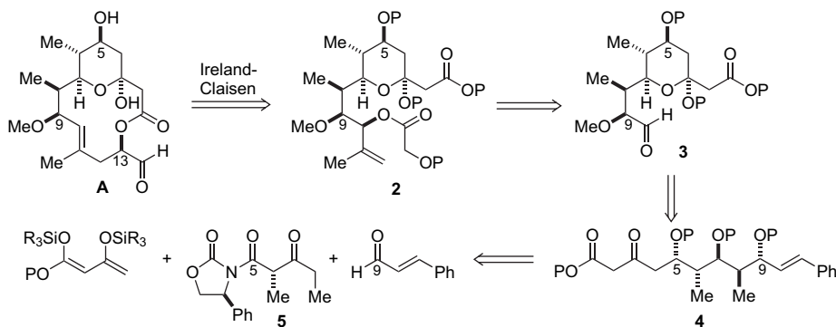
Scheme 2. First-generation retrosynthetic plan for macrolactone fragment.
