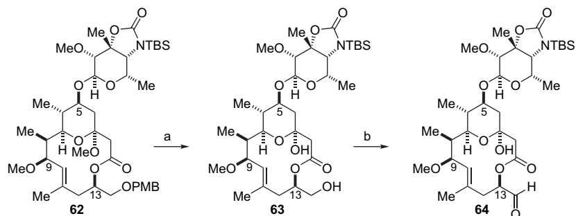
Scheme 20. Reaction conditions: (a) DDQ, CH 2 Cl 2 , MeOH, H 2 O, 83%; (b) SO 3 ·Py, Et 3 N, DMSO, CH 2 Cl 2 , 0 °C to rt.
