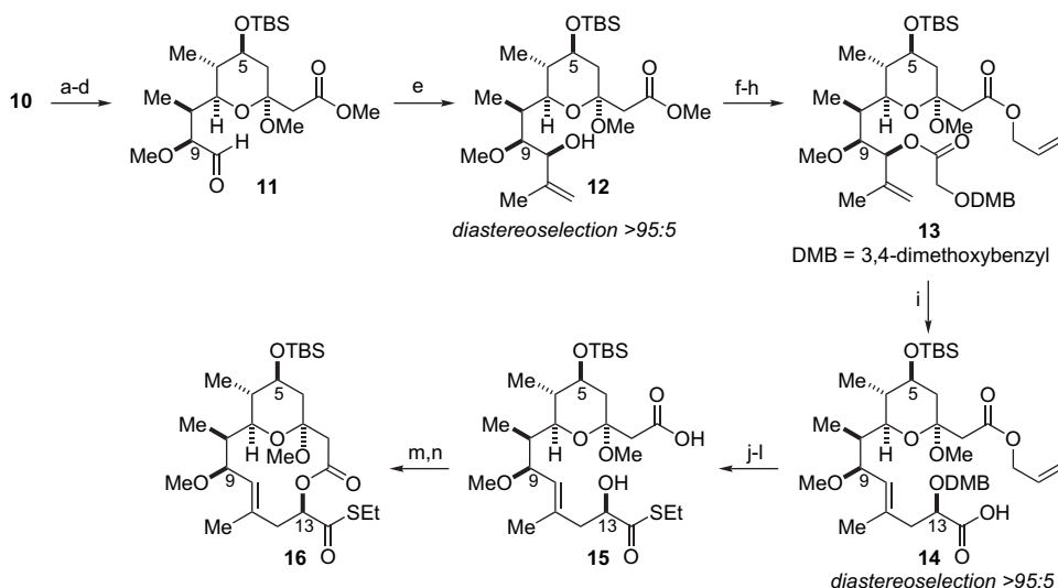
Scheme 4. Reaction conditions: (a) \text{TBSOTf} , 2,6-lutidine, \text{CH}_2\text{Cl}_2 , -78 °C; (b) PPTS, MeOH, rt, 67% (two steps); (c) \text{MeOTf} , DTBMP, \text{CH}_2\text{Cl}_2 , rt, 82%; (d) \text{O}_3 , \text{CH}_2\text{Cl}_2 , MeOH, -78 °C, then \text{Me}_2\text{S} , rt, 82%; (e) isopropenylmagnesium bromide, THF, -78 °C, 79%; (f) \text{LiOH} , MeOH, THF, \text{H}_2\text{O} , rt; (g) \text{Cs}_2\text{CO}_3 , allyl bromide, DMF, rt, 77% (two steps); (h) \text{DMBOCH}_2\text{COOH} , DCC, \text{CH}_2\text{Cl}_2 , 0 °C, then DMAP, rt, 90%; (i) \text{LiHMDS} , \text{TMSCl} \cdot \text{Et}_3\text{N} , THF, -100 °C to rt, 61%; (j) \text{EtSH} , \text{BOPCl} , \text{Et}_3\text{N} , \text{CH}_2\text{Cl}_2 , 0 °C to rt, 63%; (k) DDQ, MeOH, rt, 79%; (l) \text{Pd}(\text{PPh}_3)_4 , \text{HCO}_2\text{H} , \text{Et}_3\text{N} , THF, rt, 60%; (m) 2,4,6- \text{Cl}_3\text{C}_6\text{H}_2\text{COCl} , \text{Pr}_2\text{NEt} , THF, rt, then DMAP, toluene, 70 °C; (n) PPTS, MeOH, rt, 59% (two steps).
