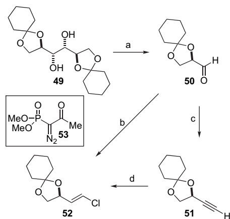
Scheme 16. Reaction conditions: (a) KIO 4 , KHCO 3 , THF/H 2 O, rt; (b) CrCl 2 , CHCl 3 , THF, 70 °C, <40% (from 49 ), 87:13 E/Z ; (c) 53 , K 2 CO 3 , MeOH, 94% (from 49 ); (d) (i) Si 2 BH, THF, −15 to 0 °C, THF; (ii) CuCl 2 , H 2 O, HMPT, THF, 0–70 °C, 70%, >20:1 E/Z .
