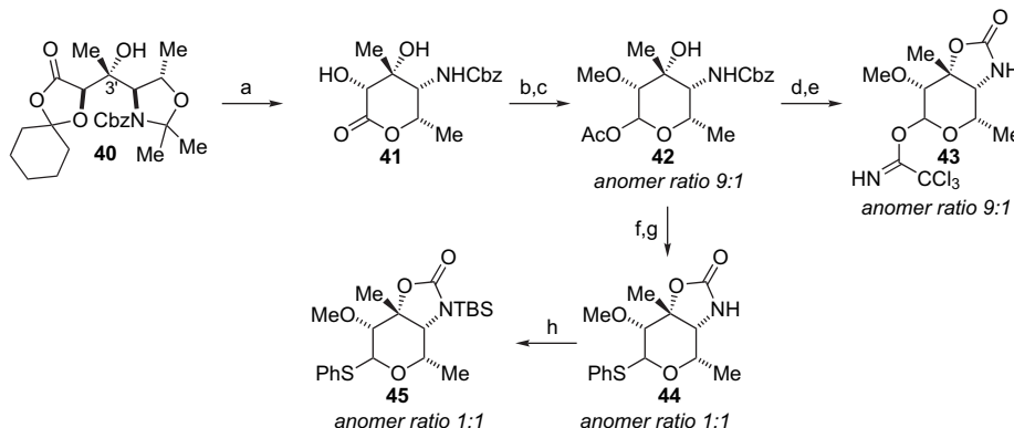
Scheme 14. Reaction conditions: (a) AcOH, 71%; (b) Me 3 O·BF 4 , DTBMP, CH 2 Cl 2 , rt, 82%; (c) DIBAL-H, CH 2 Cl 2 , Ac 2 O, DMAP, Py, 93%; (d) NaH, THF; (e) DBU, Cl 3 CCN, 51% (two steps); (f) BF 3 ·OEt 2 , PhSH, CH 2 Cl 2 , 81%; (g) NaH, THF, 97%; (h) TBSOTf, 2,6-lutidine, CH 2 Cl 2 , 92%.
