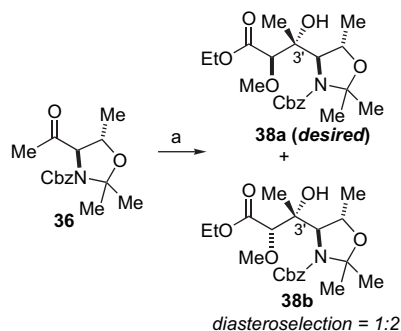
Scheme 12. Reaction conditions: (a) MeOCH 2 CO 2 Et, LDA, THF, −78 °C, 56%.
