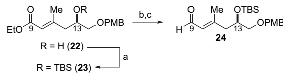
Scheme 6. Reaction conditions: (a) TBSCl, imid, DMF, rt; (b) LiAlH 4 , Et 2 O, 0 °C to rt; (c) SO 3 ·Py, Et 3 N, DMSO, CH 2 Cl 2 , 0 °C, 75% (three steps).
