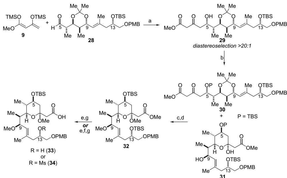
Scheme 9. Reaction conditions: (a) \text{BF}_3 \cdot \text{OEt}_2 , toluene, -90^\circ\text{C} , 88%; (b) TBSOTf, 2,6-lutidine, \text{CH}_2\text{Cl}_2 , -78^\circ\text{C} , 88%, 1.1:1 30/31 ; (c) PPTS, MeOH, rt, 91%; (d) MeOTf, DTBP, \text{CH}_2\text{Cl}_2 , rt, then PPTS, MeOH, rt, 63%; (e) TBAF, THF, rt; (f) MsCl, \text{Et}_3\text{N} , DMAP, \text{CH}_2\text{Cl}_2 , 0^\circ\text{C} ; (g) LiOH, \text{H}_2\text{O} , THF, rt, 70% (two steps for 33 ) or 68% (three steps for 34 ).
