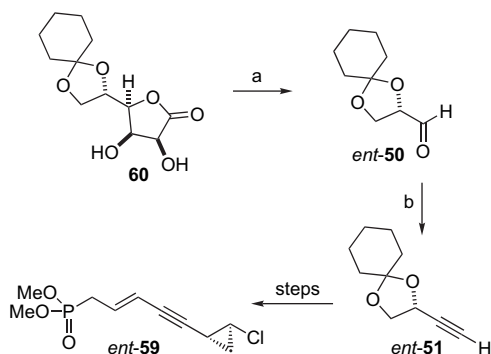
Scheme 19. Reaction conditions: (a) KIO 4 , KHCO 3 , THF/H 2 O, rt; (b) 53 , K 2 CO 3 , MeOH, rt, 77% (two steps).
