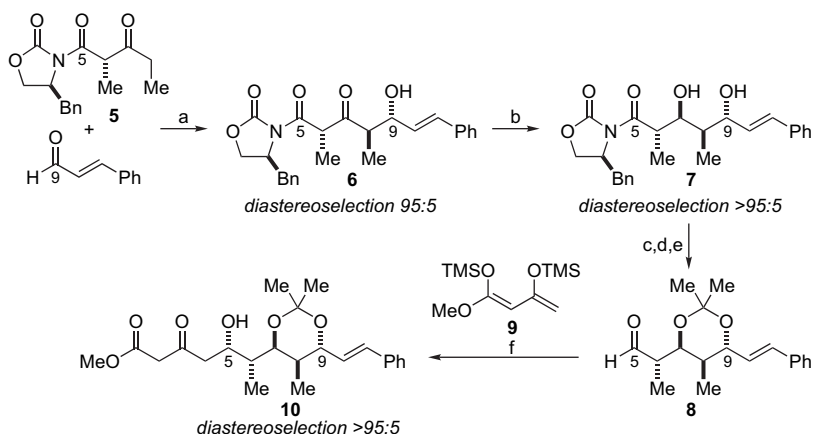
Scheme 3. Reaction conditions: (a) \text{Cy}_2\text{BCl} , \text{EtNMe}_2 , -78 to -20 °C, 78%; (b) \text{Me}_4\text{NBH}(\text{OAc})_3 , \text{AcOH} , \text{CH}_3\text{CN} , 0 °C, 98%; (c) (\text{MeO})_2\text{CMe}_2 , PPTS, acetone, rt; (d) \text{LiSEt} , THF, -5 to 0 °C; (e) DIBAL-H, toluene, -78 °C, 66% (three steps); (f) \text{BF}_3 \cdot \text{OEt}_2 , toluene, -78 °C, 86%.
