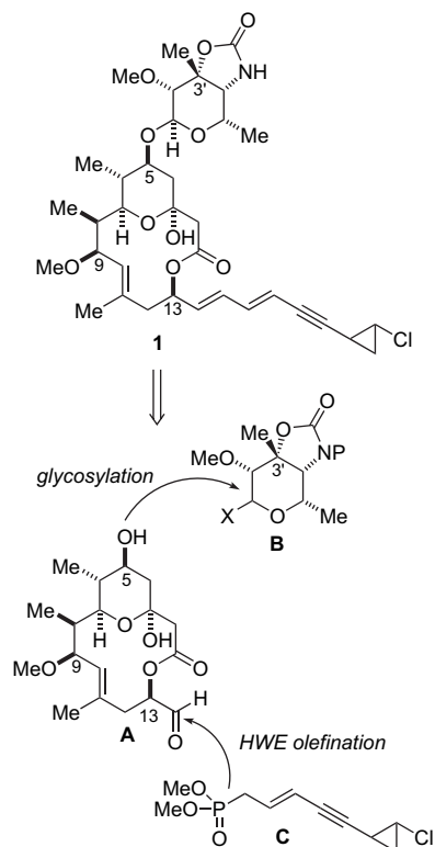
Scheme 1. General synthesis strategy.
