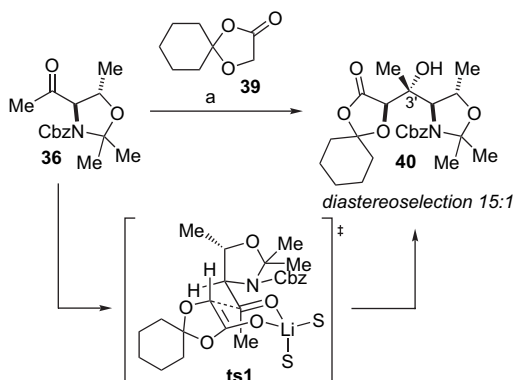
Scheme 13. Reaction conditions: (a) LDA, THF, −50 °C, 89%.
