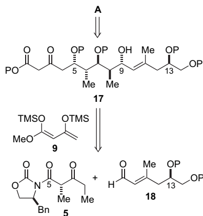
Scheme 5. Second-generation retrosynthetic plan for macrolactone fragment.
