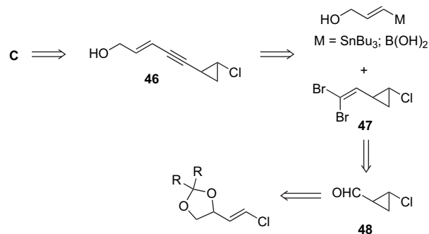
Scheme 15. Strategy for the construction of the side chain fragment.
