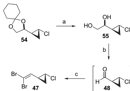
Scheme 17. Reaction conditions: (a) Dowex resin, MeOH, rt, 82%; (b) Pb(OAc) 4 , K 2 CO 3 , CH 2 Cl 2 , rt; (c) PPh 3 , CBr 4 , CH 2 Cl 2 , 94% (two steps).
