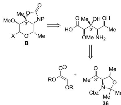
Scheme 10. Retrosynthetic analysis of callipeltose.
