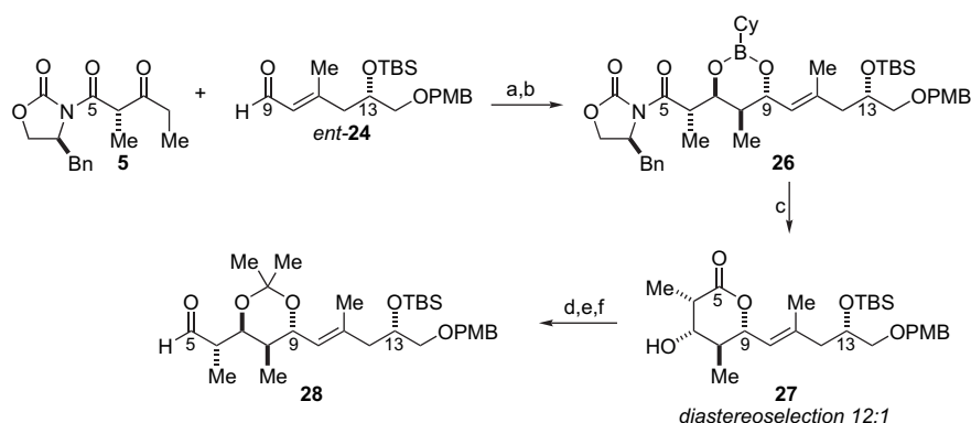
Scheme 8. Reaction conditions: (a) 5 , \text{Cy}_2\text{BCl} , \text{EtNMe}_2 , 0^\circ\text{C} , then ent - 24 , -78^\circ\text{C} ; (b) \text{Me}_4\text{NB}(\text{OAc})_3 , \text{MeCN} , \text{AcOH} , 0^\circ\text{C} ; (c) \text{HN}(\text{CH}_2\text{CH}_2\text{OH})_2 , \text{EtOAc} , rt, 86% (three steps); (d) \text{HNMe}(\text{OMe})\cdot\text{HCl} , \text{AlMe}_3 , \text{CH}_2\text{Cl}_2 , 0^\circ\text{C} to rt; (e) \text{Me}_2\text{C}(\text{OMe})_2 , PPTS, acetone, rt; (f) \text{LiAlH}_4 , \text{Et}_2\text{O} , rt, 72% (three steps).
