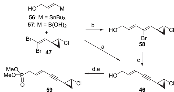
Scheme 18. Reaction conditions: (a) 56 , 2.5 mol % Pd 2 dba 2 , 15 mol % P( p -C 6 H 4 OMe) 3 , i Pr 2 NEt, <50%; (b) 10 mol % Pd(PPh 3 ) 4 , TIOEt, THF/H 2 O, rt, 93%; (c) DBU, toluene, 110 °C, 99%; (d) CBr 4 , PPh 3 , CH 2 Cl 2 , −40 °C, 94%; (e) P(OMe) 3 , 100 °C, 80%.
