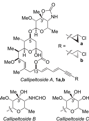
Figure 1. The structures of callipeltosides A–C.
