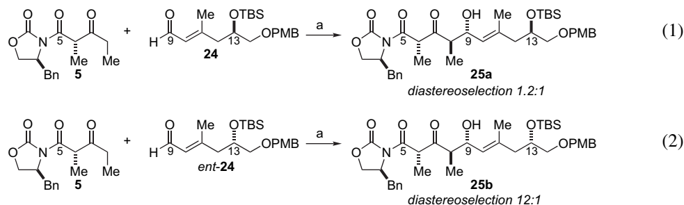
Scheme 7. Reaction conditions: (a) 5 , \text{Cy}_2\text{BCl} , \text{EtNMe}_2 , \text{Et}_2\text{O} , 0^\circ\text{C} , \text{RCHO} , -78^\circ\text{C} .
